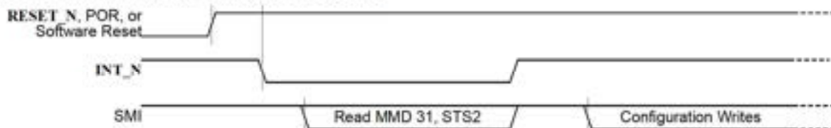
Figure 4-3. Initialization and Configuration Sequence
