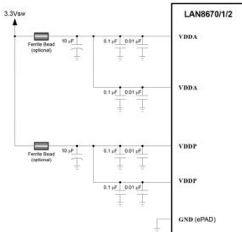
Figure 6-3. Power Connectivity
