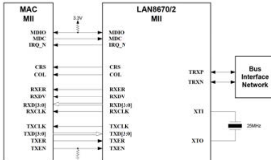
Figure 6-1. MII Connectivity
