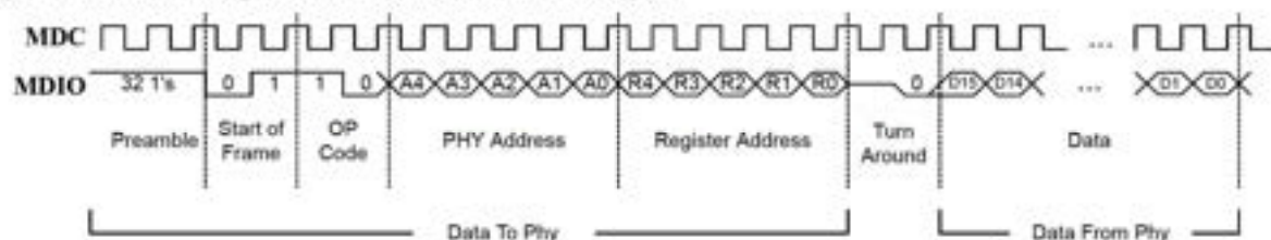
Figure 4-1. SMI Timing and Frame Structure - READ Cycle
